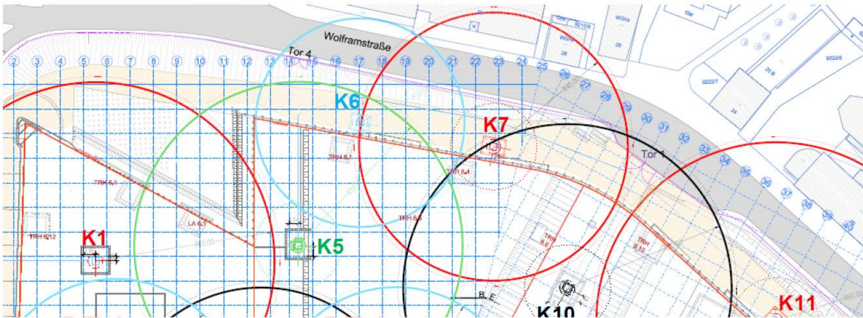
Izvor: Buildings: Characteristics of Equipment Planning for Multi-Crane Building Construction Sites (Aavid Shapira and Albert Ben-David, 2017. god. Faculty of Civil and Environmental Engineering, Technion–Israel Institute of Technology)
